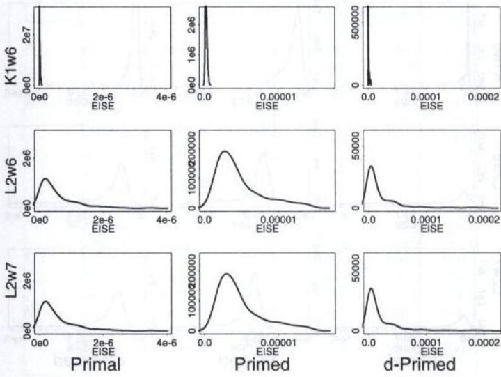
Model A - The fourth moment.
