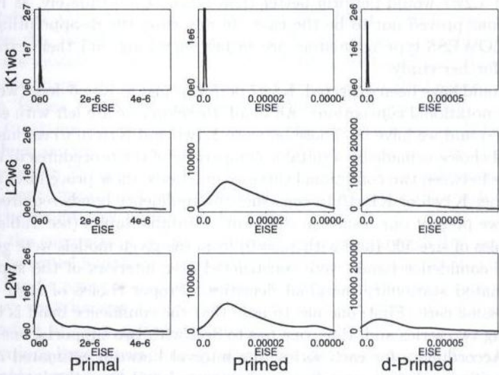
Model B - The fourth moment.
